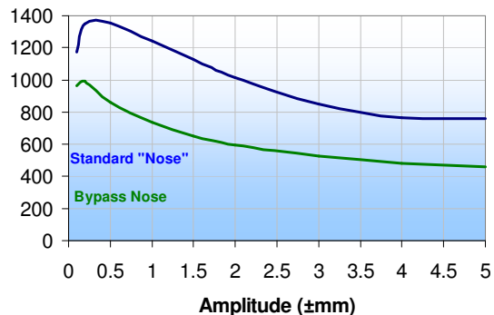
Dynamic Stiffness at 15Hz Y Direction
