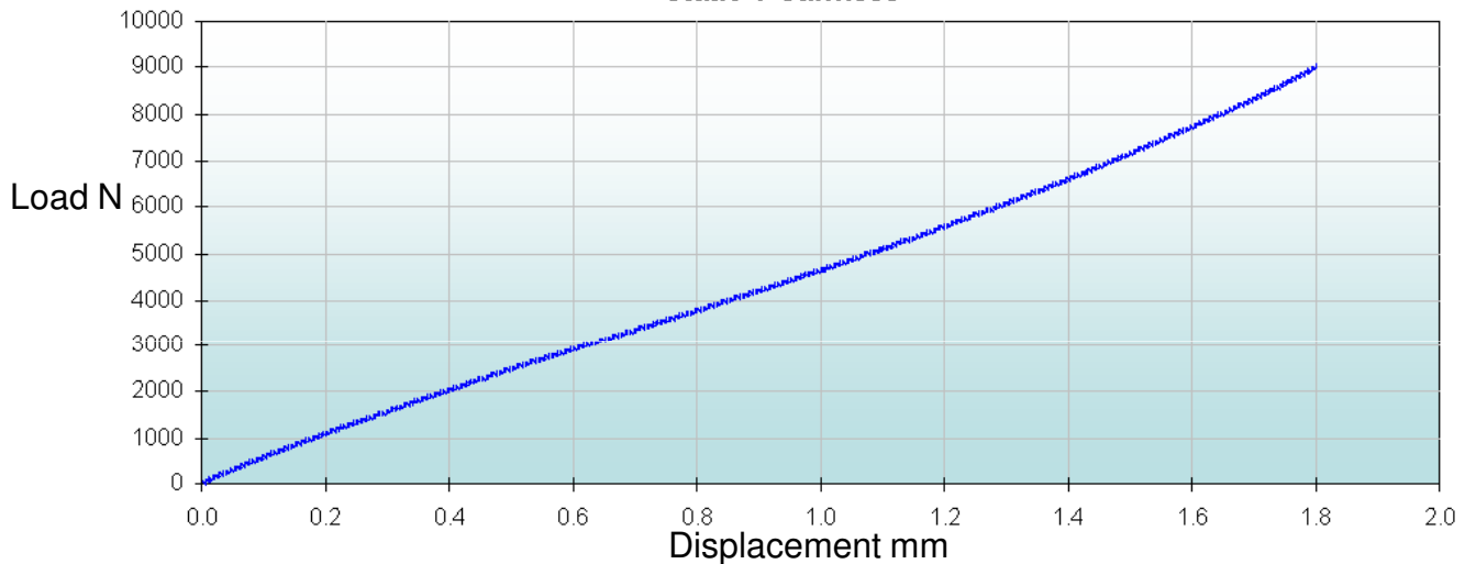
Static Y Stiffness
