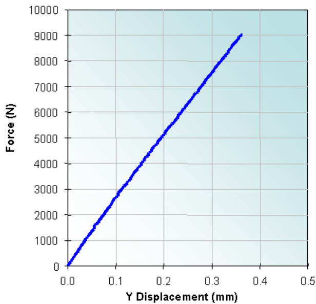
Static Y Stiffness
