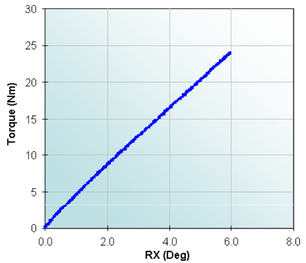
Static RX Stiffness
