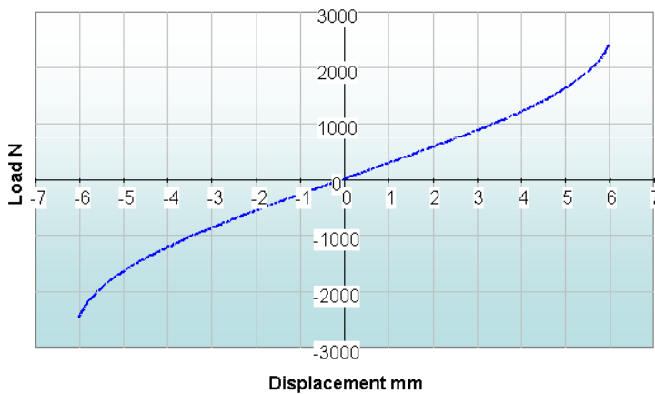
AXIAL RATES
